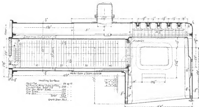
Fig. 5113. Water Tube Locomotive Boiler. London & South Western.
